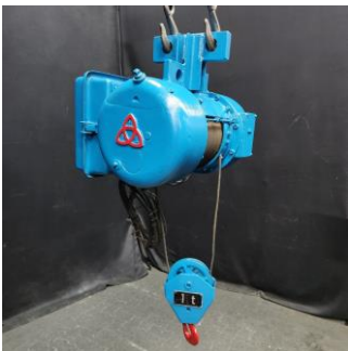
1Ton Lash Hoist
