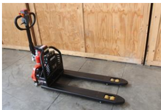
1500kg Electric Pallet Jack - CBD15J with Li-ion Battery and Charger
